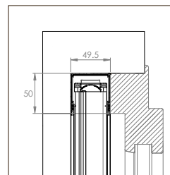
EVA INCAS SR MIDI
