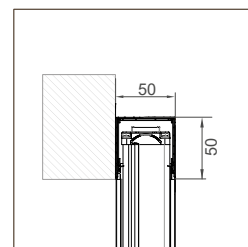
EVA UP MIDI 50/50
