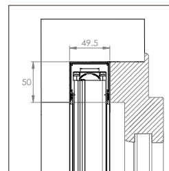
EVA INCAS MIDI 35/35
