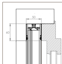
EVA INCAS STANDARD 50/35
