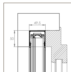
EVA INCAS MIDI 20/20
