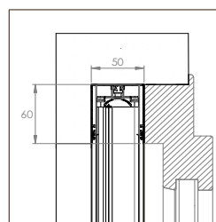
EVA INCAS STANDARD 50/50
