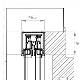
AURORAPLUS INCAS MIDI
