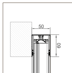
EVA UP STANDARD 50/50
