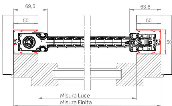
AURORAPLUS INCAS STANDARD
