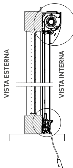
APPL. STANDARD (FIG. 1)
