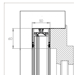
■ EVA INCAS STANDARD 50/50
