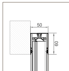
EVA UP STANDARD 35/35
