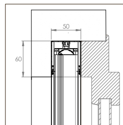
EVA INCAS STANDARD 35/35
