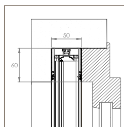
EVA INCAS STANDARD 20/20
