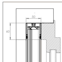
EVA INCAS SR STANDARD
