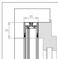
EVA INCAS STANDARD 20/20
