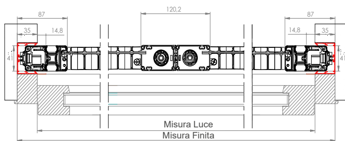
EVA INCAS STANDARD 35/35
