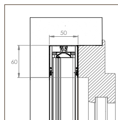
EVA INCAS STANDARD 50/20
