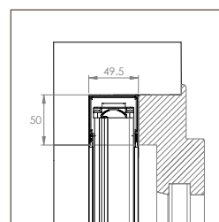
EVA INCAS MIDI 20/20
